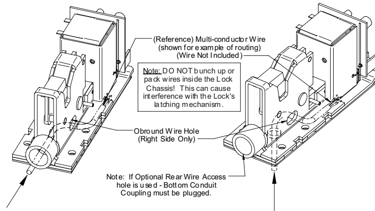
Figure 9 – Wire Routing
