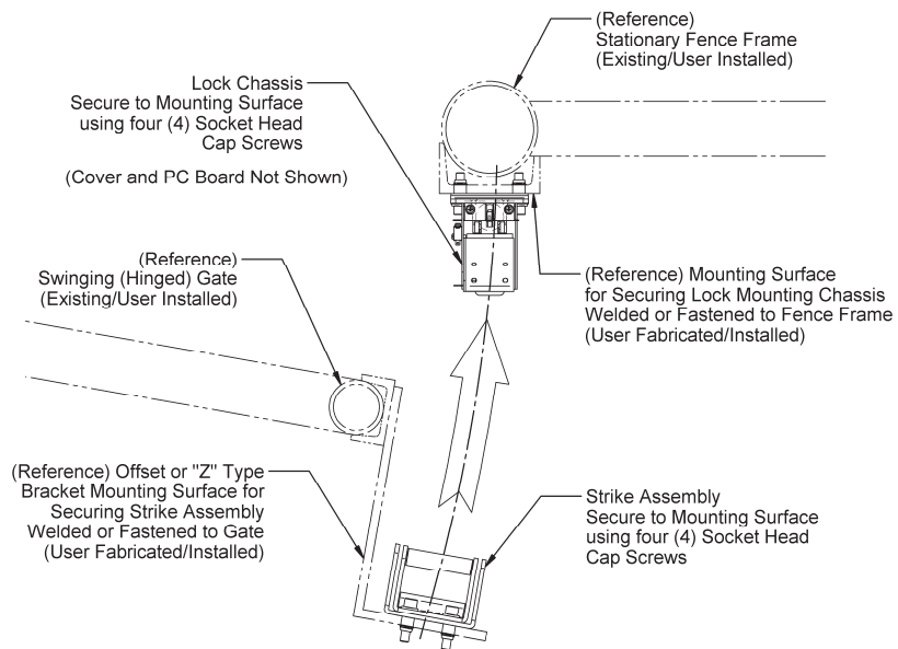
Figure 1 – Swing Gate Operation
